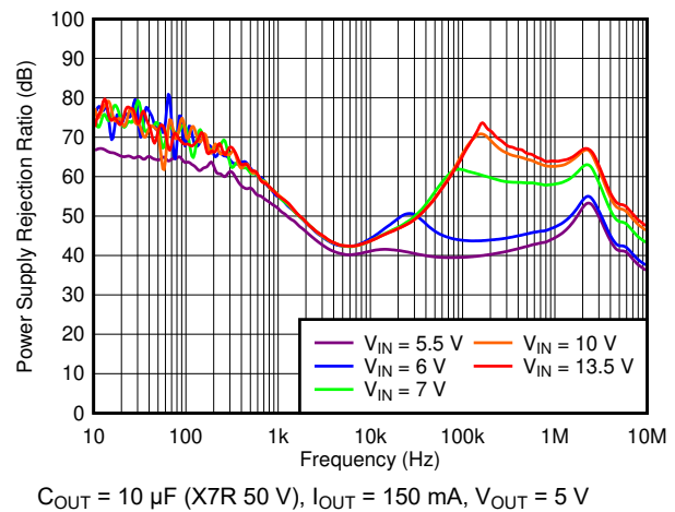
图 6-10. PSRR vs Frequency and V_{IN}
