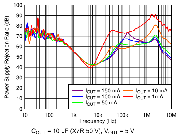
图 6-9. PSRR vs Frequency and I_{OUT}
