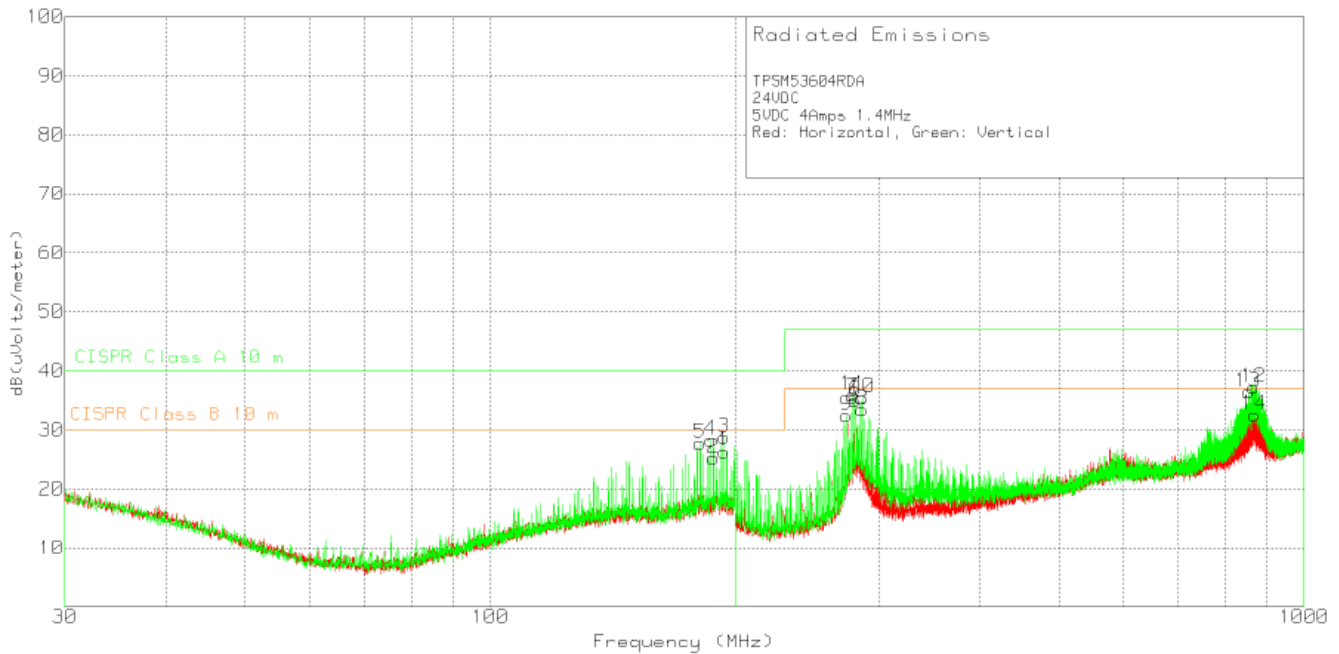
图 10-5. Radiated Emissions 24-V Input, 5-V Output, 4-A Load
