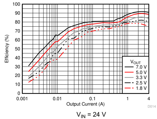
图 6-14. Efficiency versus Output Current
