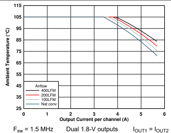
图 6-13. Safe Operating Area ( V_{OUT} = 1.8\text{ V} )
