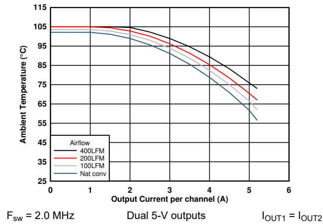
6-7. Safe Operating Area ( V_{OUT} = 5 \text{ V} )
