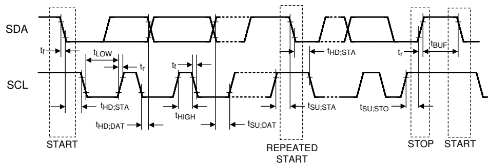
图 6-2. I²C Serial Control Bus Timing
