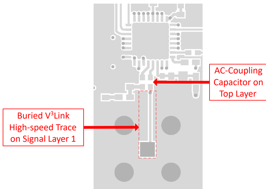
图 10-1. TSER953 Serializer DOUT+ Trace Layout
