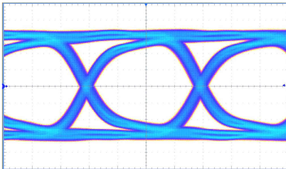
图 6-3. Eye Diagram at 4-Gbps V³Link Forward Channel Rate From Serializer Output
