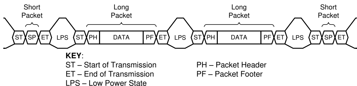
图 7-1. CSI-2 Protocol Layer With Short and Long Packets
