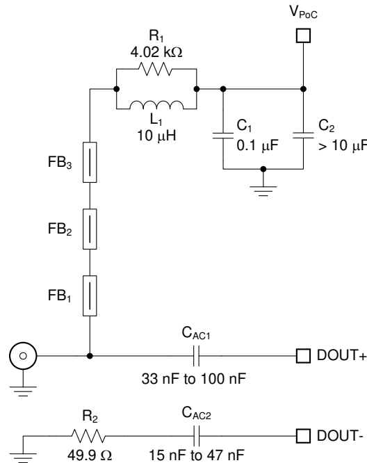
图 8-2. Typical PoC Network for a "4G" V³Link
