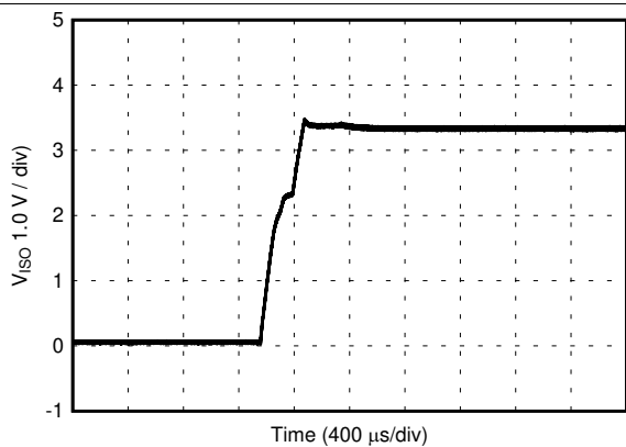
图 51. V_{ISO} Soft Start at 10% Rated Load, 5.0-V Input, 3.3-V Output
