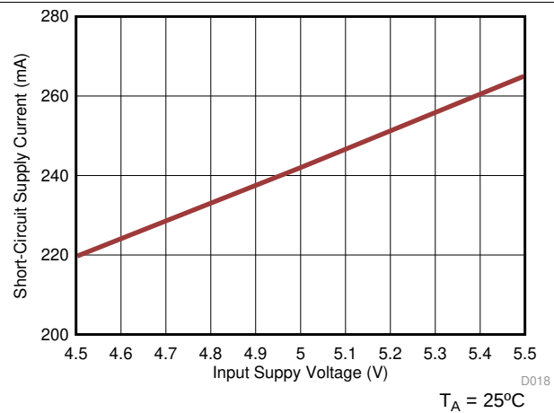
图 24. Short-Circuit Supply Current ( I_{INP\_SC} ) vs Supply Voltage ( V_{INP} )
