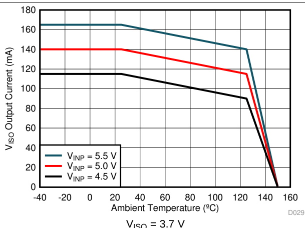
图 11. Maximum V_{ISO} Output Current vs. Temperature
