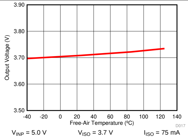
图 23. Isolated Supply Voltage ( V_{ISO} ) vs Free-Air Temperature
