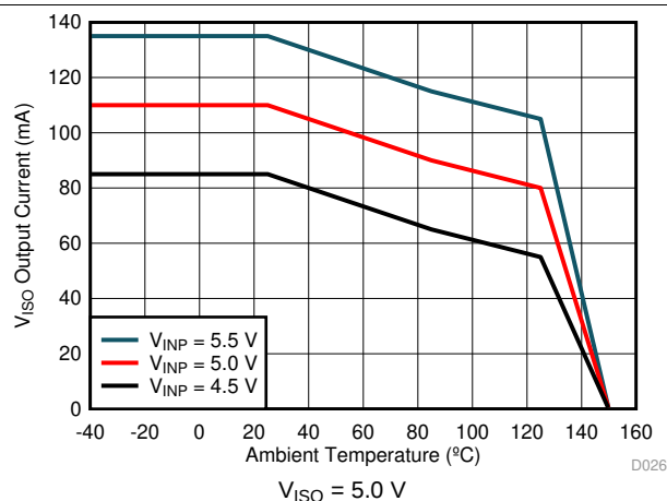
图 8. Maximum V_{ISO} Output Current vs. Temperature
