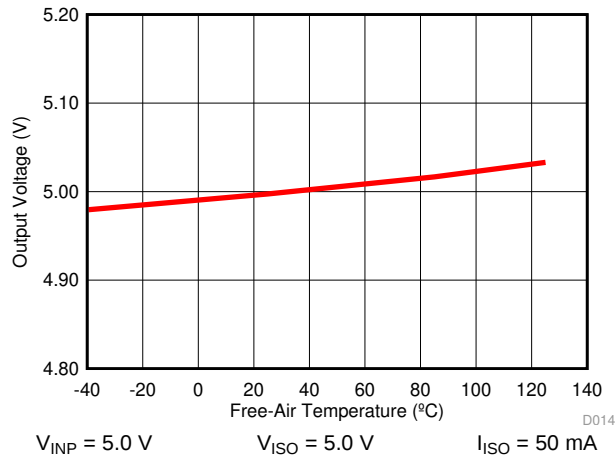
图 20. Isolated Supply Voltage ( V_{ISO} ) vs Free-Air Temperature
