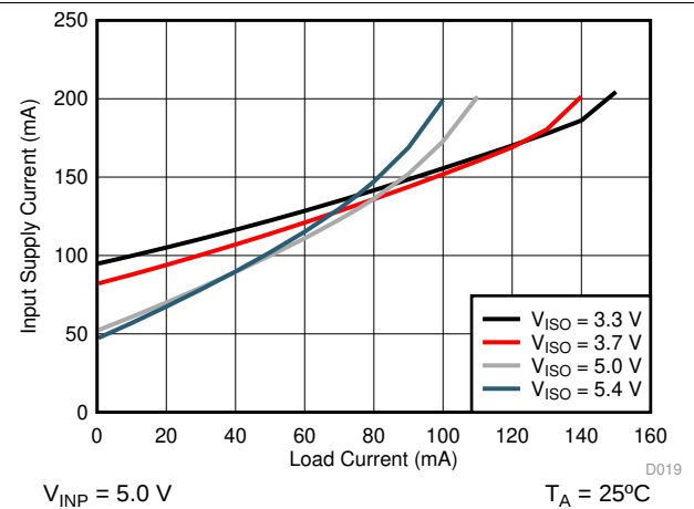
图 25. Input Supply Current ( I_{INP} ) vs Load Current ( I_{ISO} )
