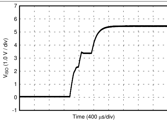
图 45. V_{ISO} Soft Start at 10% Rated Load, 5.0-V Input, 5.4-V Output
