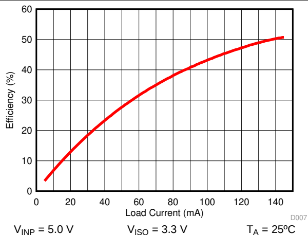
图 14. Power Supply Efficiency vs Load Current ( I_{ISO} )
