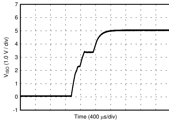
图 48. V_{ISO} Soft Start at 90% Rated Load, 5.0-V Input, 5.0-V Output
