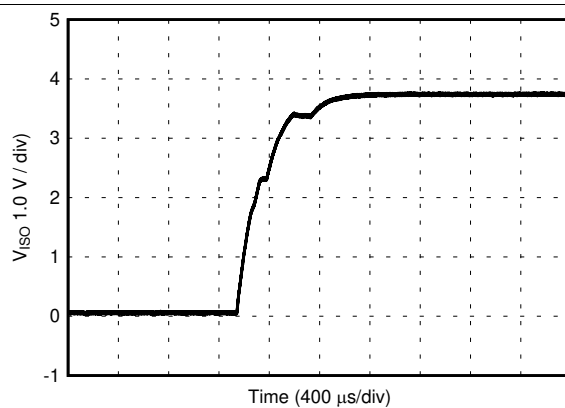
图 50. V_{ISO} Soft Start at 90% Rated Load, 5.0-V Input, 3.7-V Output
