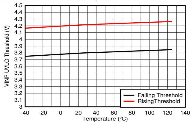
图 26. Typical V_{INP} UVLO Threshold vs Junction Temperature ( T_J )
