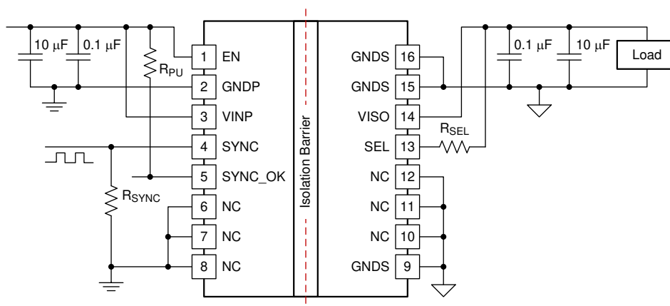
图 28. Typical Application
