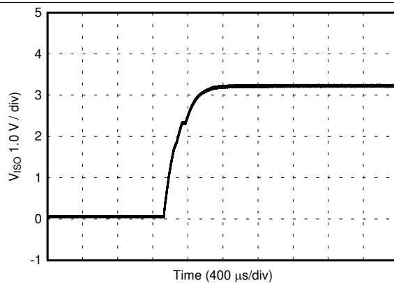
图 52. V_{ISO} Soft Start at 90% Rated Load, 5.0-V Input, 3.3-V Output
