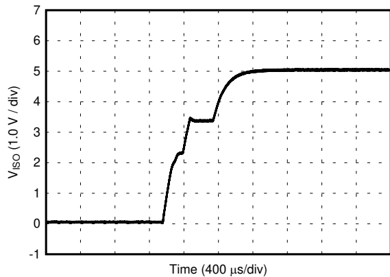
图 47. V_{ISO} Soft Start at 10% Rated Load, 5.0-V Input, 5.0-V Output
