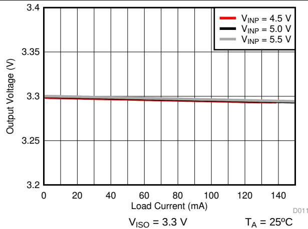
图 18. Isolated Supply Voltage ( V_{ISO} ) vs Load Current ( I_{ISO} )
