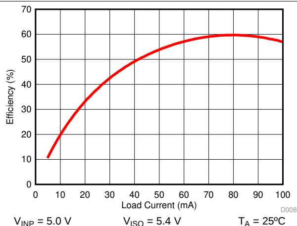
图 13. Power Supply Efficiency vs Load Current ( I_{ISO} )
