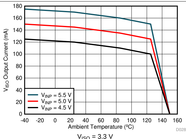
图 10. Maximum V_{ISO} Output Current vs. Temperature
