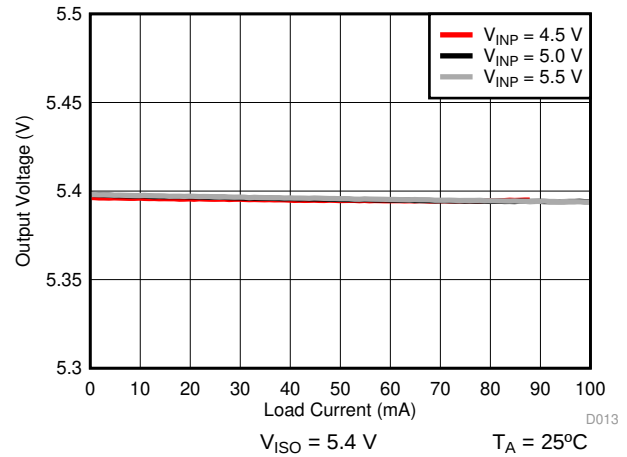
图 17. Isolated Supply Voltage ( V_{ISO} ) vs Load Current ( I_{ISO} )
