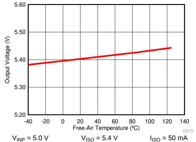
图 21. Isolated Supply Voltage ( V_{ISO} ) vs Free-Air Temperature
