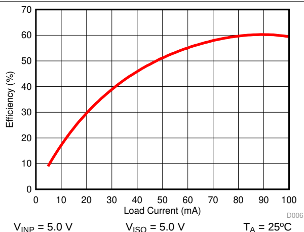
图 12. Power Supply Efficiency vs Load Current ( I_{ISO} )
