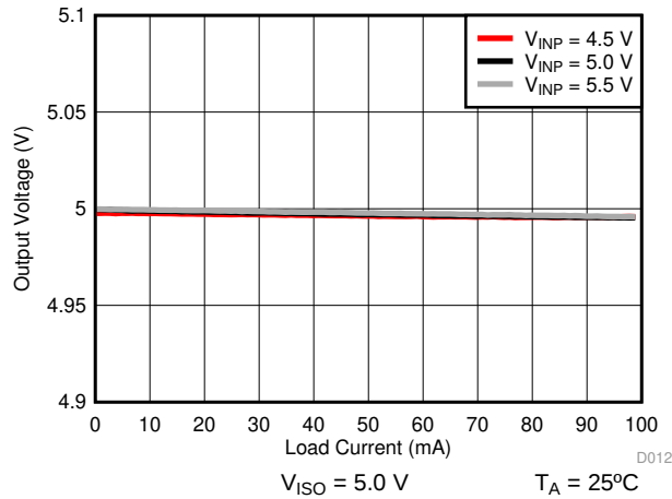
图 16. Isolated Supply Voltage ( V_{ISO} ) vs Load Current ( I_{ISO} )
