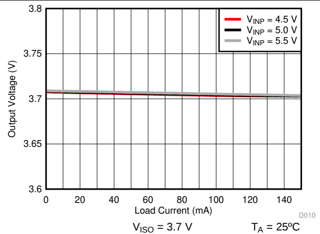
图 19. Isolated Supply Voltage ( V_{ISO} ) vs Load Current ( I_{ISO} )
