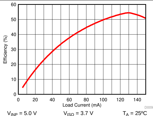
图 15. Power Supply Efficiency vs Load Current ( I_{ISO} )
