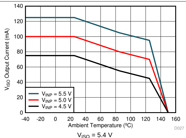
图 9. Maximum V_{ISO} Output Current vs. Temperature
