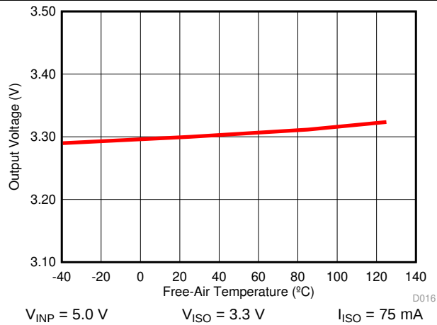
图 22. Isolated Supply Voltage ( V_{ISO} ) vs Free-Air Temperature
