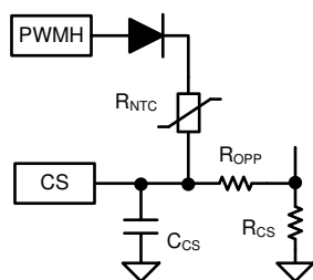
图 8-43. Two Connections to Implement OTP on the CS Pin
