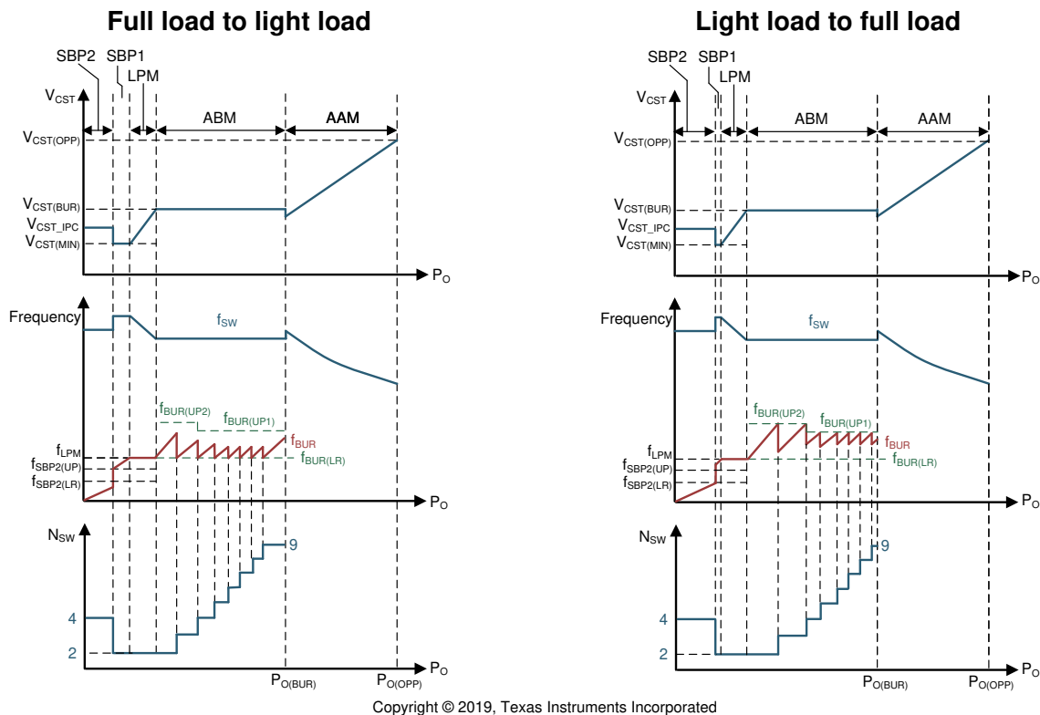
图 8-25. Control Law Under Different Load Sweep Direction as V_{IPC} > 0.9 V and V_{VS} > V_{VSLV(UP)}
