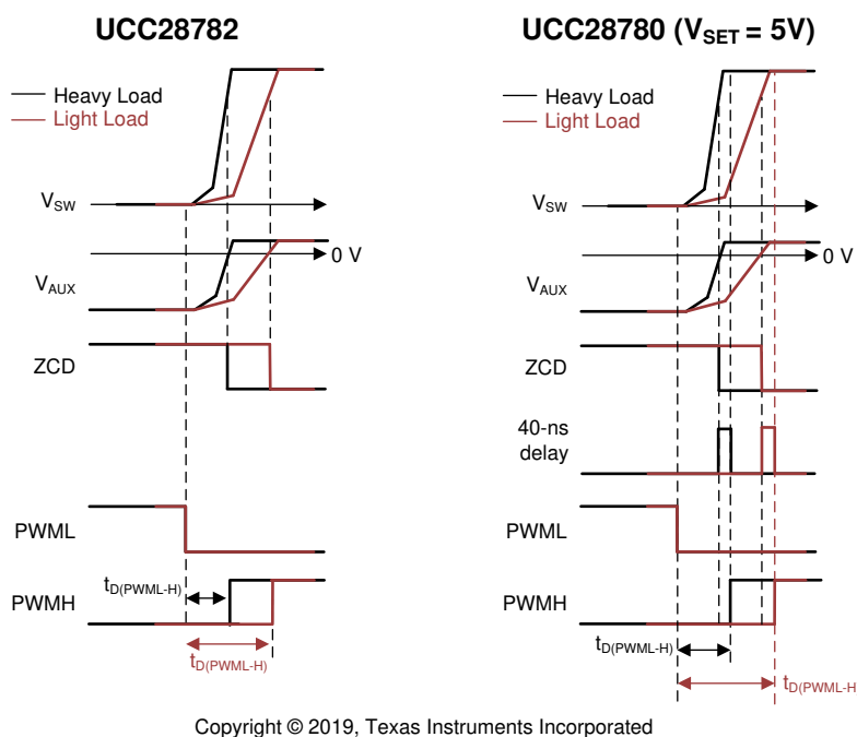
图 8-22. t_{D(PWML-H)} Control Optimized for GaN and Si FETs
