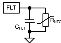
图 8-41. Two Connections to Implement OTP on the FLT Pin
