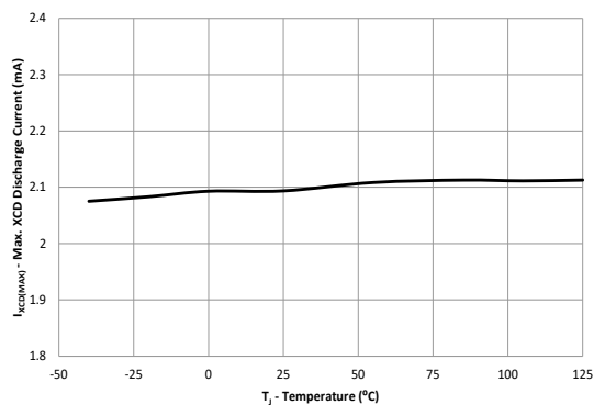
图 7-13. Max. XCD Discharge Current vs. Junction Temperature
