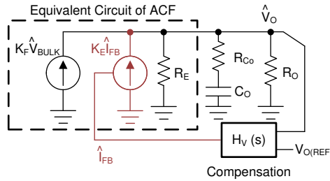
图 9-2. Small-Signal Model of ACF in AAM Loop
