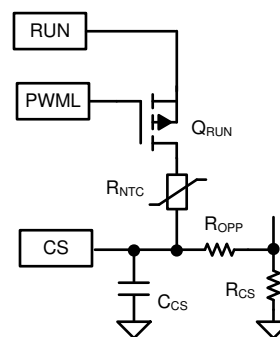
图 8-43. Two Connections to Implement OTP on the CS Pin
