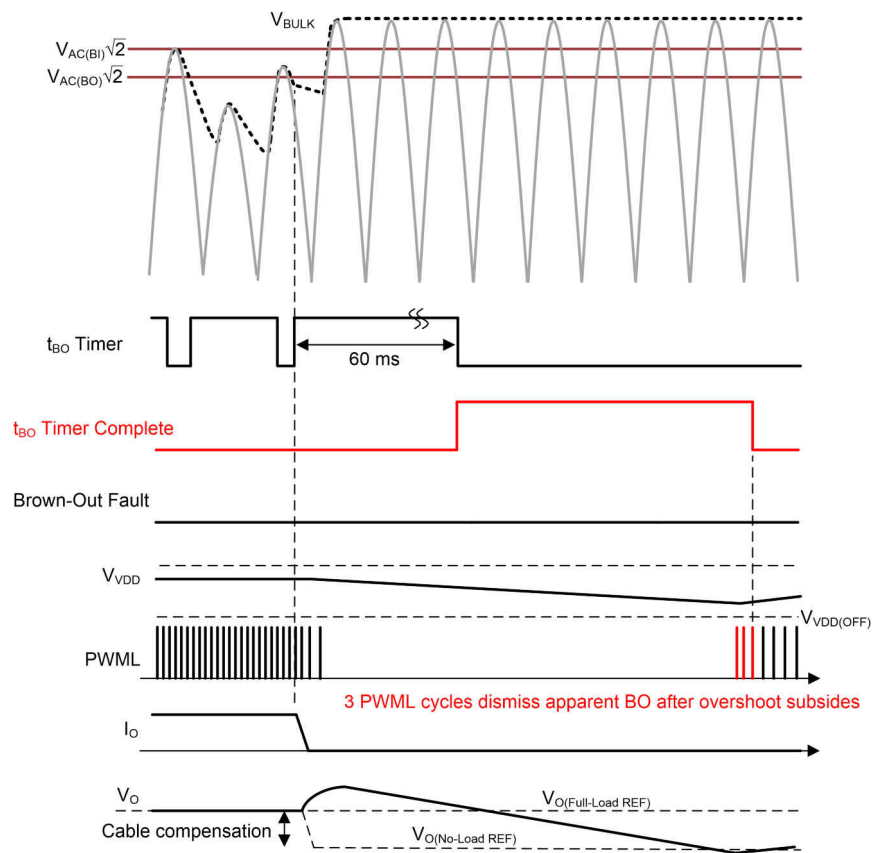
图 8-38. Timing Diagram of Brown-Out Response on Extended Output Overshoot
