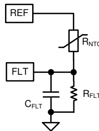
图 8-41. Two Connections to Implement OTP on the FLT Pin
