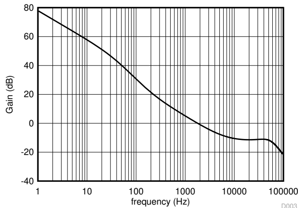
图 9-5. Converter Closed-Loop Bode Plot - Gain
