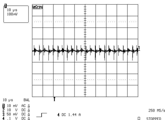
图 9-10. Output Voltage Ripple at Full Load (100 mV/div)
