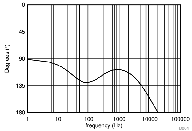
图 9-6. Converter Closed-Loop Bode Plot - Phase
