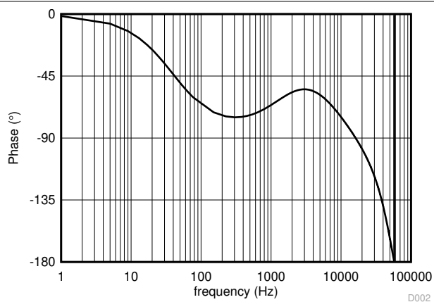
图 9-4. Converter Open-Loop Bode Plot - Phase
