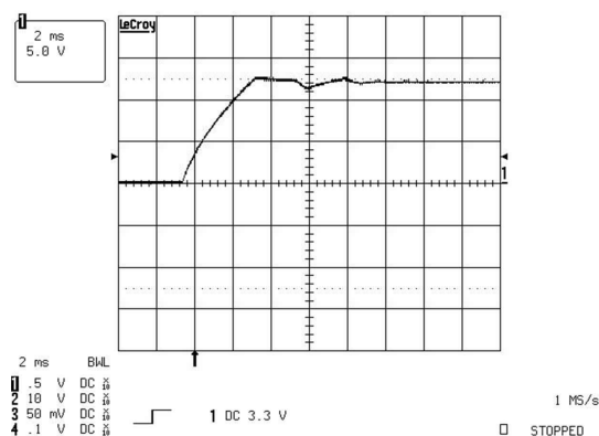
图 9-11. Output Voltage Behavior at Full Load Start-up (5 V/div)
