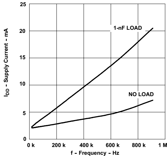
图 7-15. Supply Current vs Oscillator Frequency
