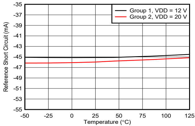
图 7-7. Reference Short-Circuit Current vs Temperature
