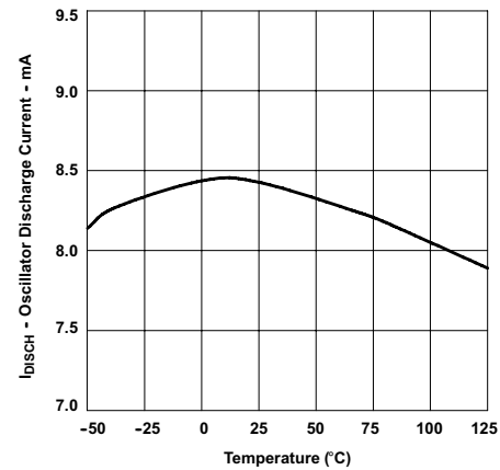
图 7-2. Oscillator Discharge Current vs Temperature
