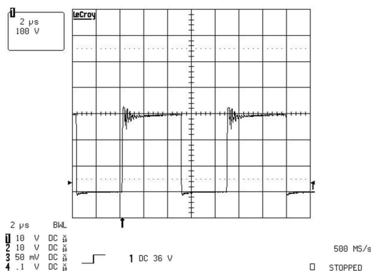
图 9-8. Primary Side MOSFET Drain-to-Source Voltage at 120-V AC Input (100 V/div)
