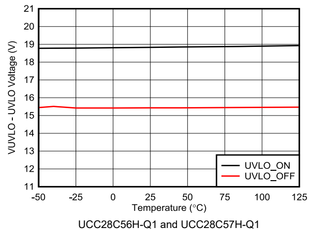
图 7-12. Undervoltage Lockout vs Temperature
