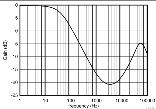
图 9-3. Converter Open-Loop Bode Plot - Gain
