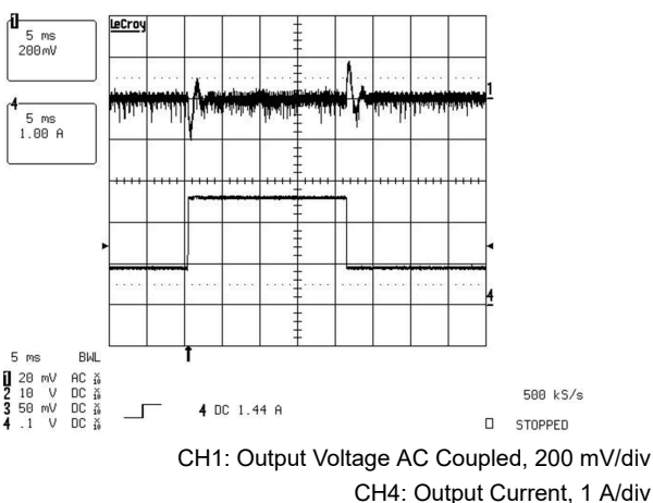
图 9-9. Output Voltage During 0.9-A to 2.7-A Load Transient
