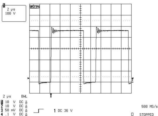
图 9-7. Primary Side MOSFET Drain-to-Source Voltage at 240-V AC Input (100 V/div)
