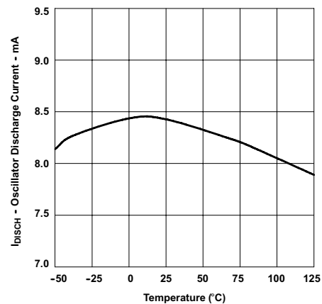
图 7-2. Oscillator Discharge Current vs Temperature
