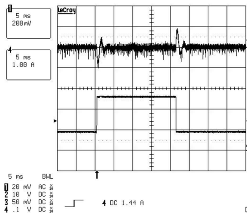
CH1: Output Voltage AC Coupled, 200 mV/div CH4: Output Current, 1 A/div
