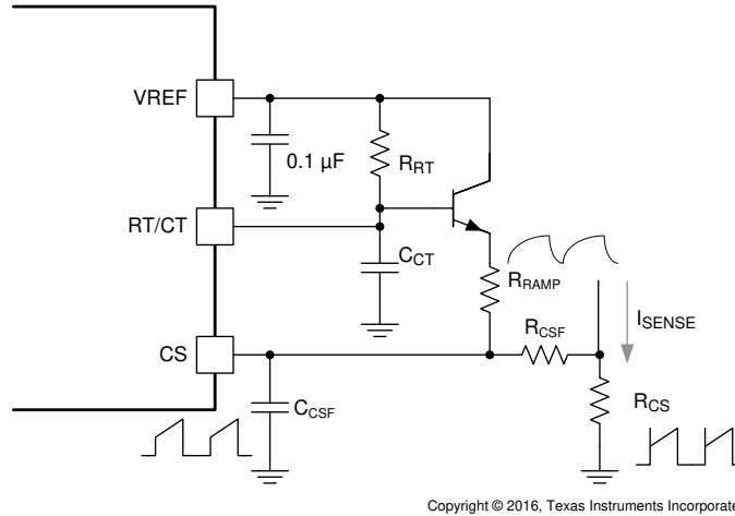
图 8-8. Slope Compensation Circuit
