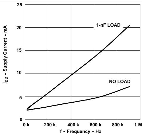
图 7-15. Supply Current vs Oscillator Frequency
