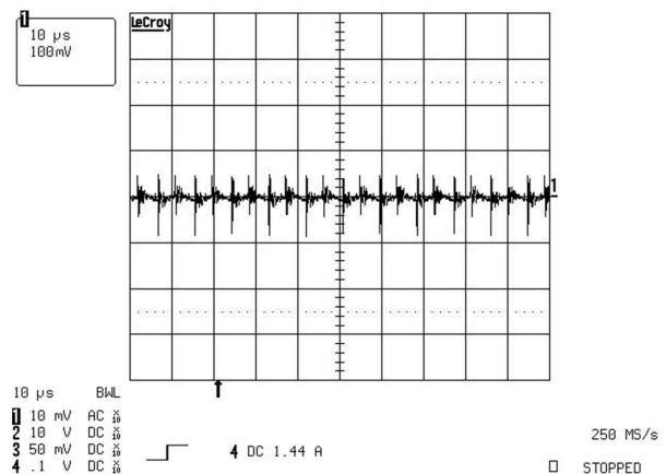
图 9-11. Output Voltage Ripple at Full Load (100 mV/div)
