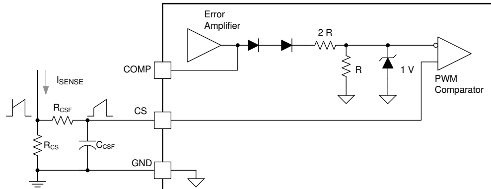
图 8-3. Current-Sense Circuit Schematic
