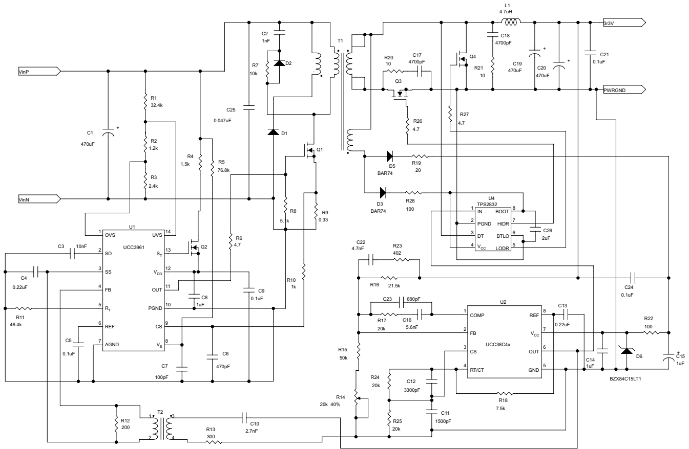
图 9-2. Forward Converter with Synchronous Rectification Using the UCC38C42 as the Secondary-Side Controller
