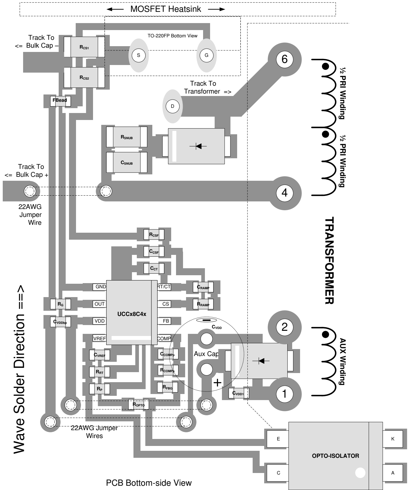
图 11-1. UCCx8C4x Layout Example
