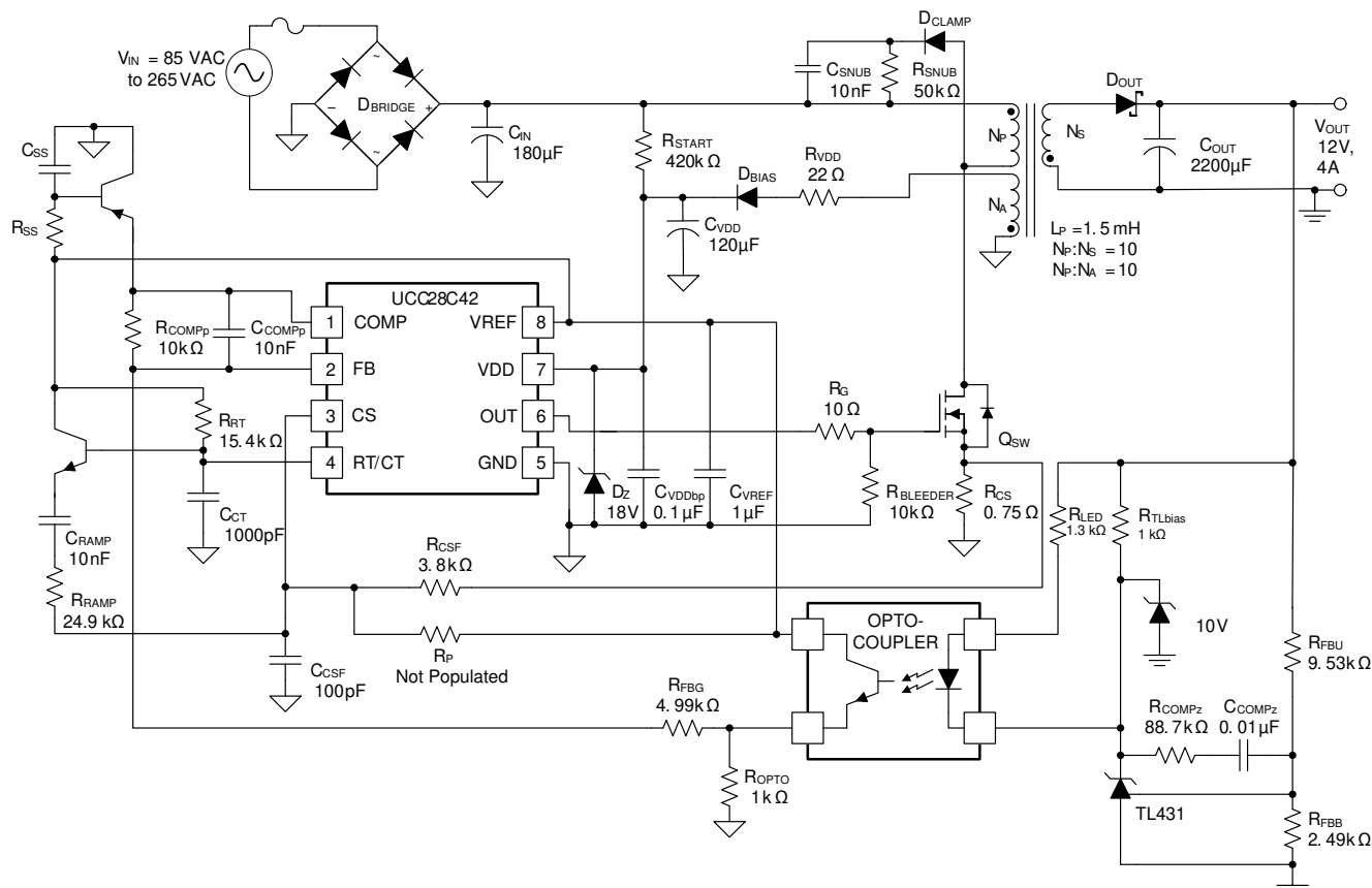
图 9-3. Typical Application Design Schematic
