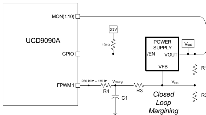
图 7-22. Closed-Loop Margining
