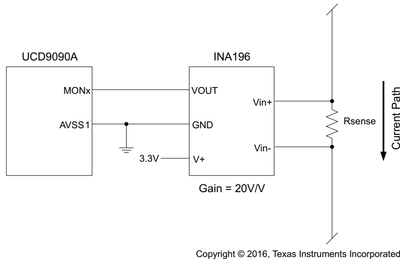
图 7-8. Current Monitoring Circuit Example Using the INA196
